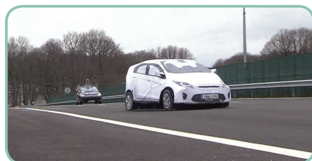
FIG 12 The vehicle dummy used in VEH use cases.
