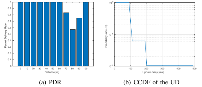
Fig. 11. Packet Delivery Rate and Complementary Cumulative Distribution Function of the Update Delay for Experiment 4 (Scenario 2).
