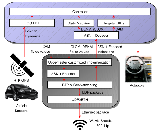
Fig. 3. Flow diagram of the communications system [12].
