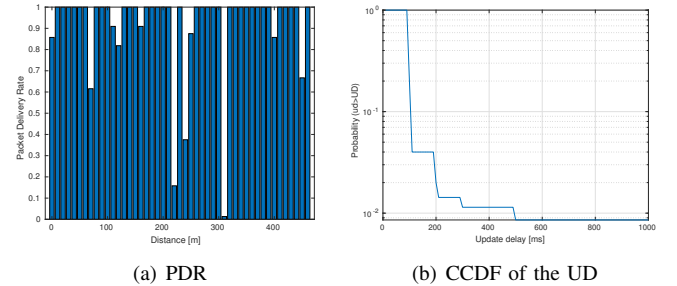
Fig. 9. Packet Delivery Rate and Complementary Cumulative Distribution Function of the Update Delay for Experiment 2 (Scenario 1).
