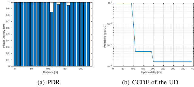
Fig. 10. Packet Delivery Rate and Complementary Cumulative Distribution Function of the Update Delay for Experiment 3 (Scenario 1).
