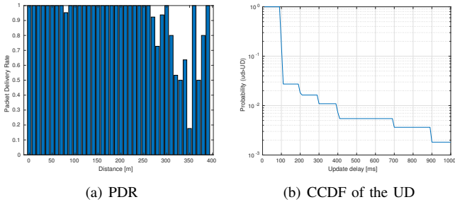
Fig. 8. Packet Delivery Rate and Complementary Cumulative Distribution Function of the Update Delay for Experiment 1 (Baseline).
