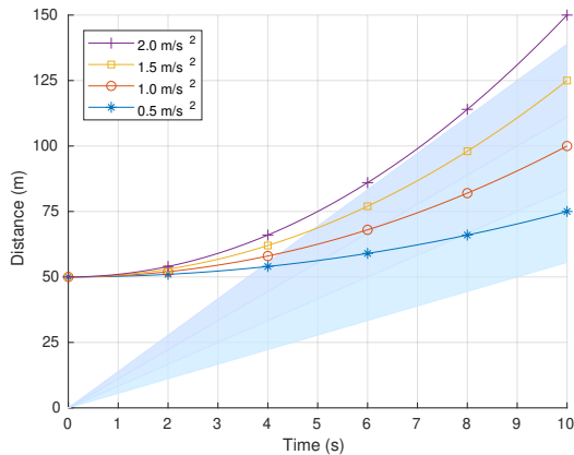
Fig. 5. Analysis of a T-intersections management. The shadowed area represents the distance run by a vehicle moving at constant speed of 20-50 Km/h. The lines represent the distance run by a second vehicle 50m ahead of the first one with a constant acceleration of 0.5-2m/s^2 .
