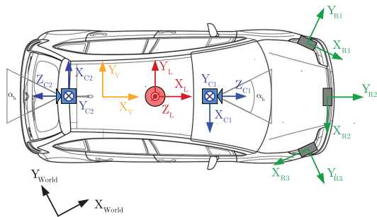
Fig. 1. DRIVERTIVE vehicle. In green the radars position, in blue the cameras position, in red the Lidar position and in yellow the RTK GPS position.
