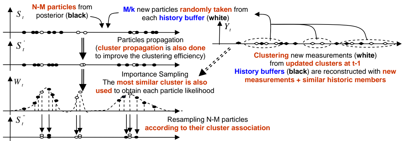
Figure 3. Description of the XPF-CP functionality
