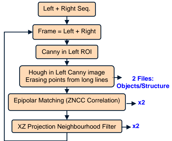
Figure 2. Block diagram of the stereo-vision classifier and object detector
