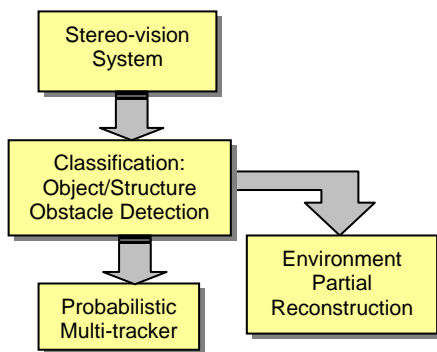
Figure 1. Block diagram of the global tracking system
